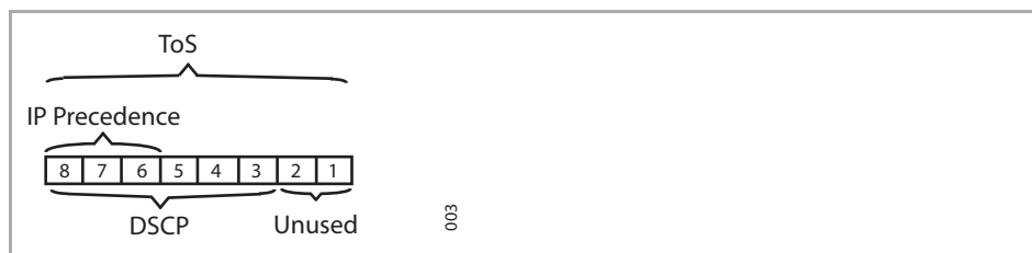
Figure 2 Diffserv Redefinition of ToS Field.
