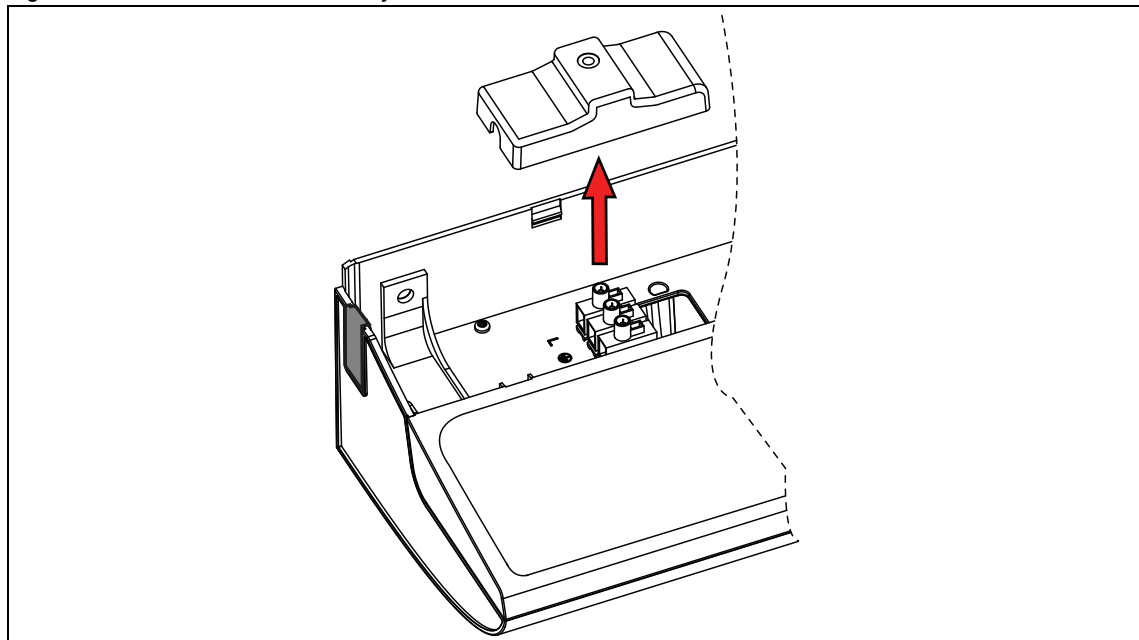
Figure 6 Remove safety cover
