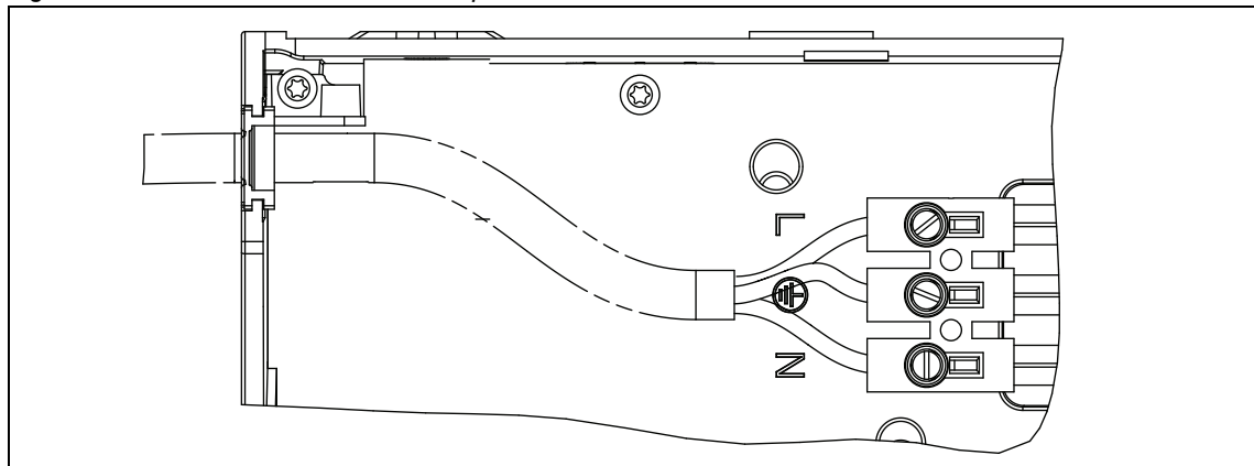
Figure 8 Terminal block for power cord
