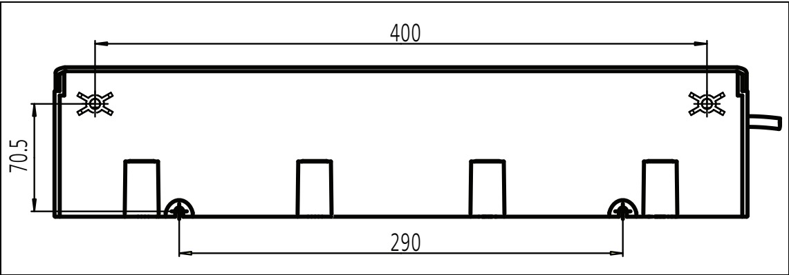
Figure 2 Mounting dimensions in mm - Charging Rack seen from back
