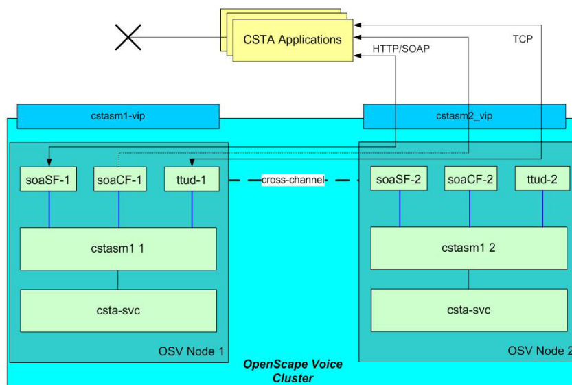
Figure 8 Connection Failure due to Network Problems
