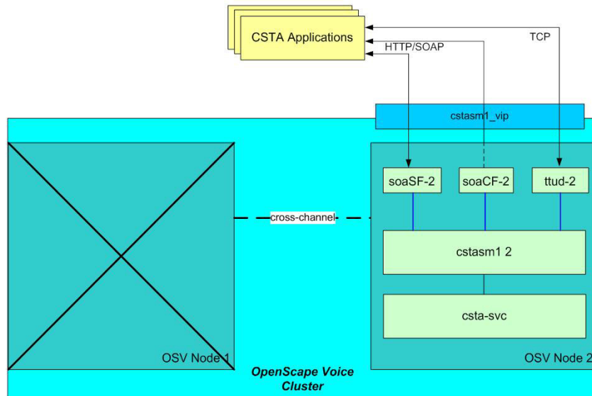
Figure 6 Co-Located Node Cluster Failover
