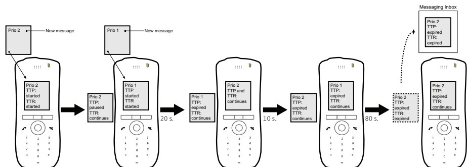
Figure 7 Message handling without manually closing a message.
