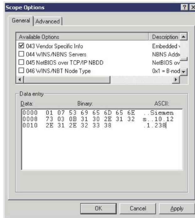
Figure 5 Option 43 using a standard DHCP vendor class.
