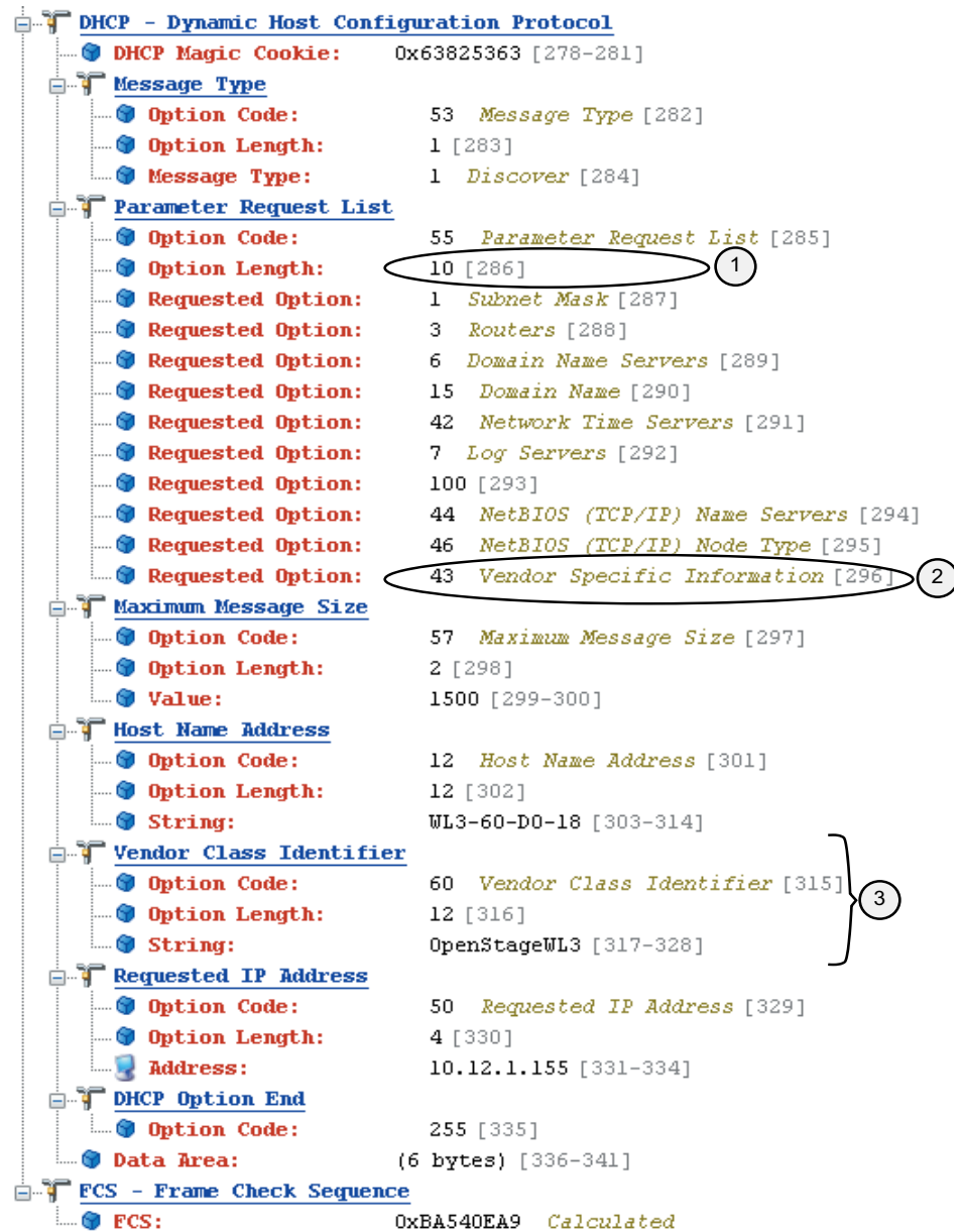
Figure 2 Example of a DHCP Discover message (Omnipeek trace).
