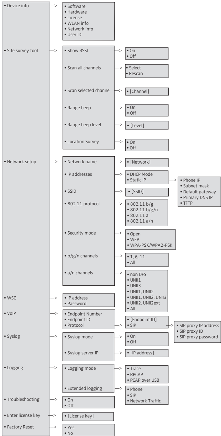
Figure 5 Admin Menu in the Handset.
